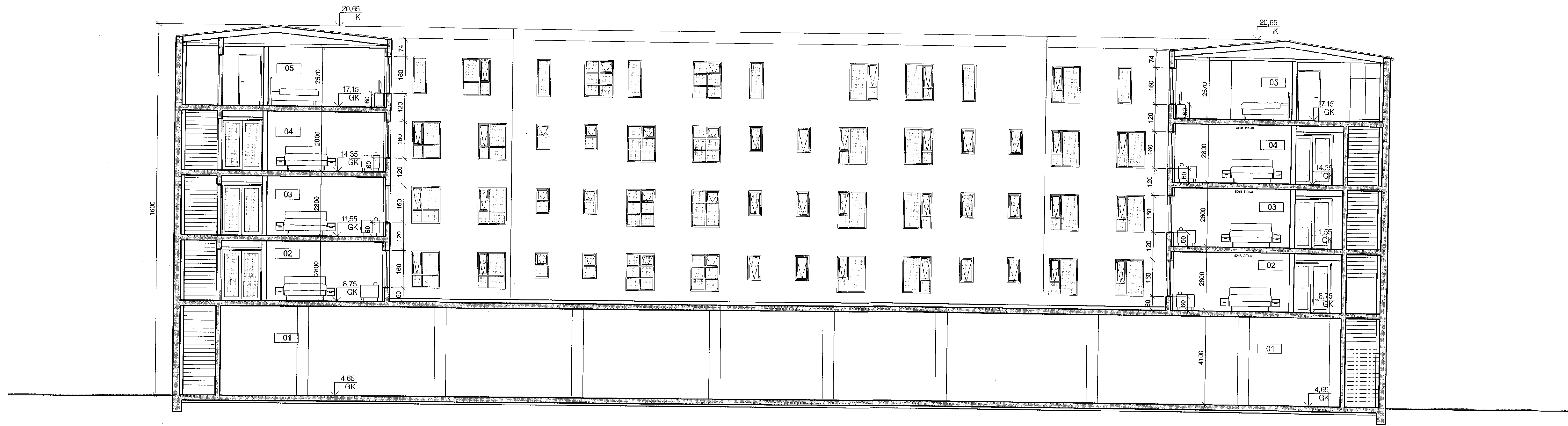
C-C 10-02 10-03 10-04 10-05 10-06 10-07 ÚTLIT/ SNID 1:100
